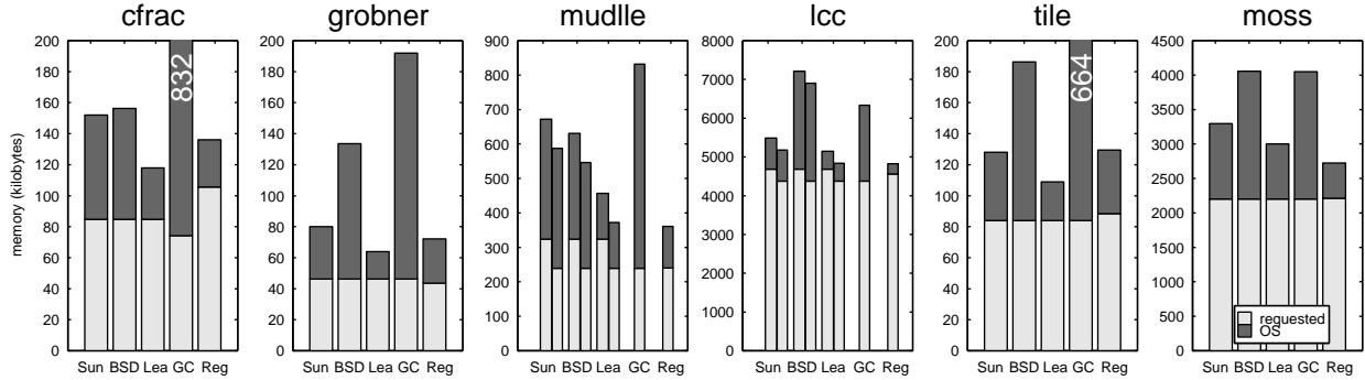
Figure 8: Memory overhead.
